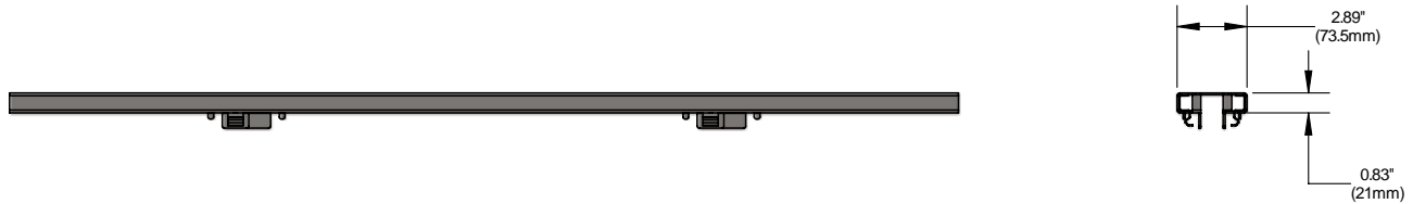
Side elevation
